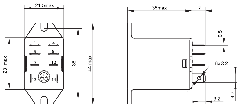
Outline Dimensions
