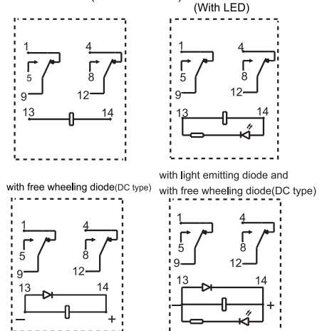
Wiring Diagram
